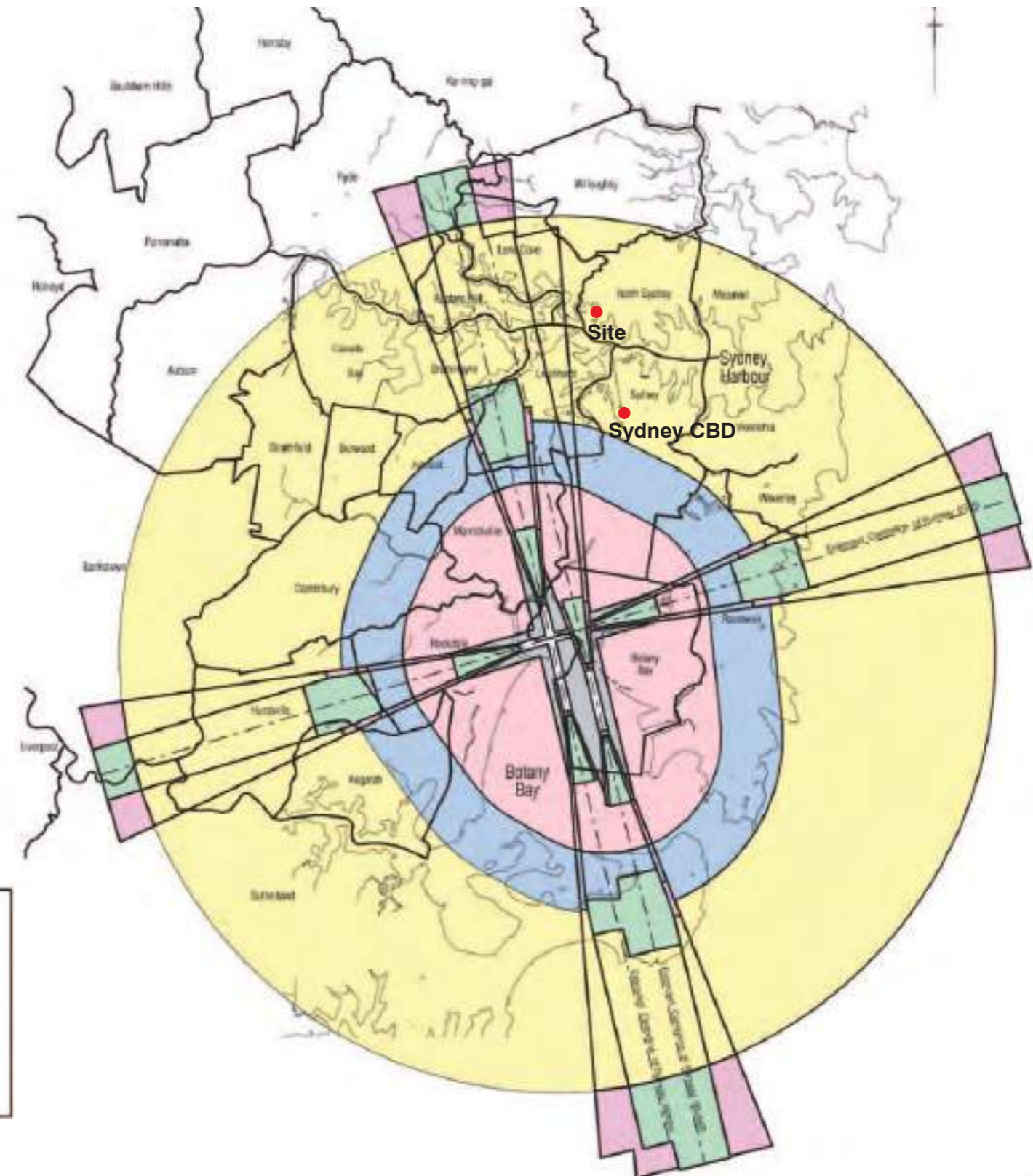
Obstacle limitation surfaces (Sydney Airport)
