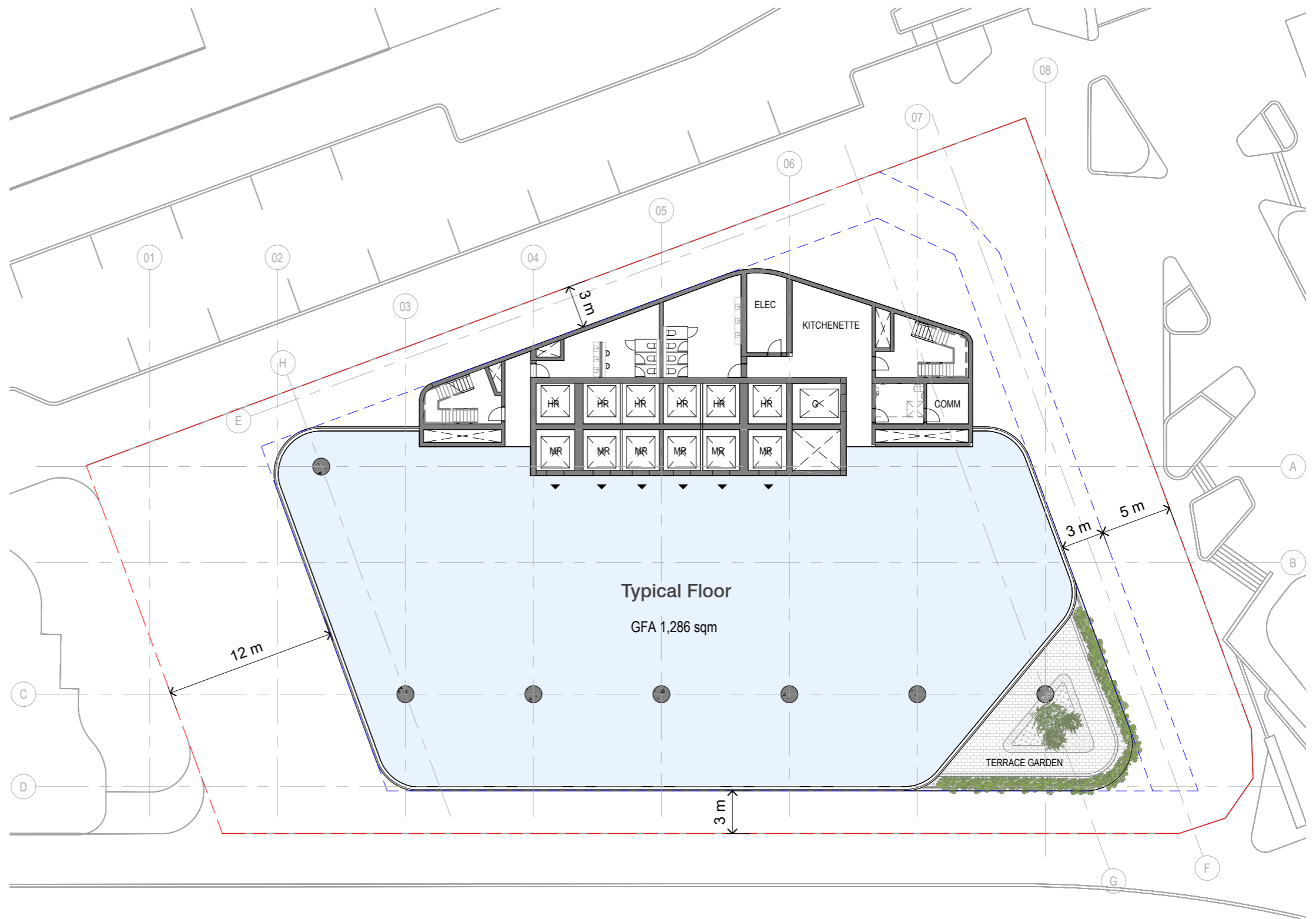
Indicative L22- special client floor plan with sky-garden
