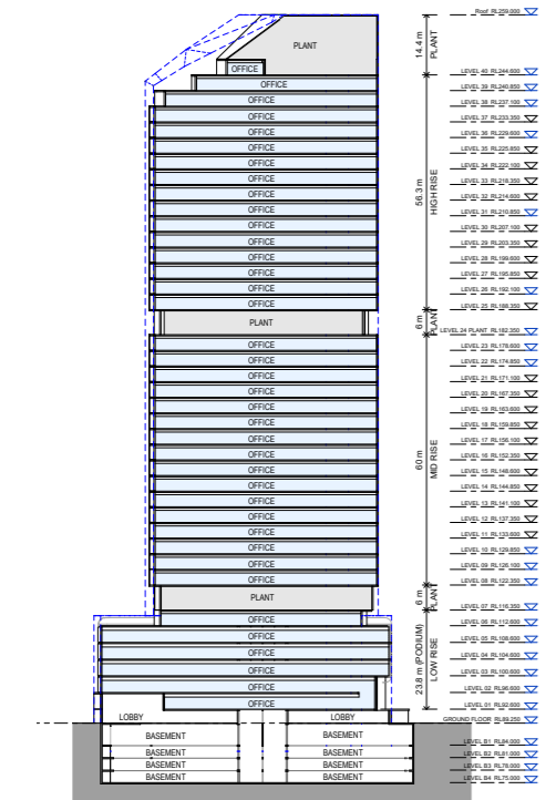
Section of the new proposal
