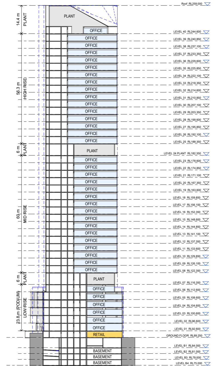
section2 showing the permissible envelope in blue dotted line
